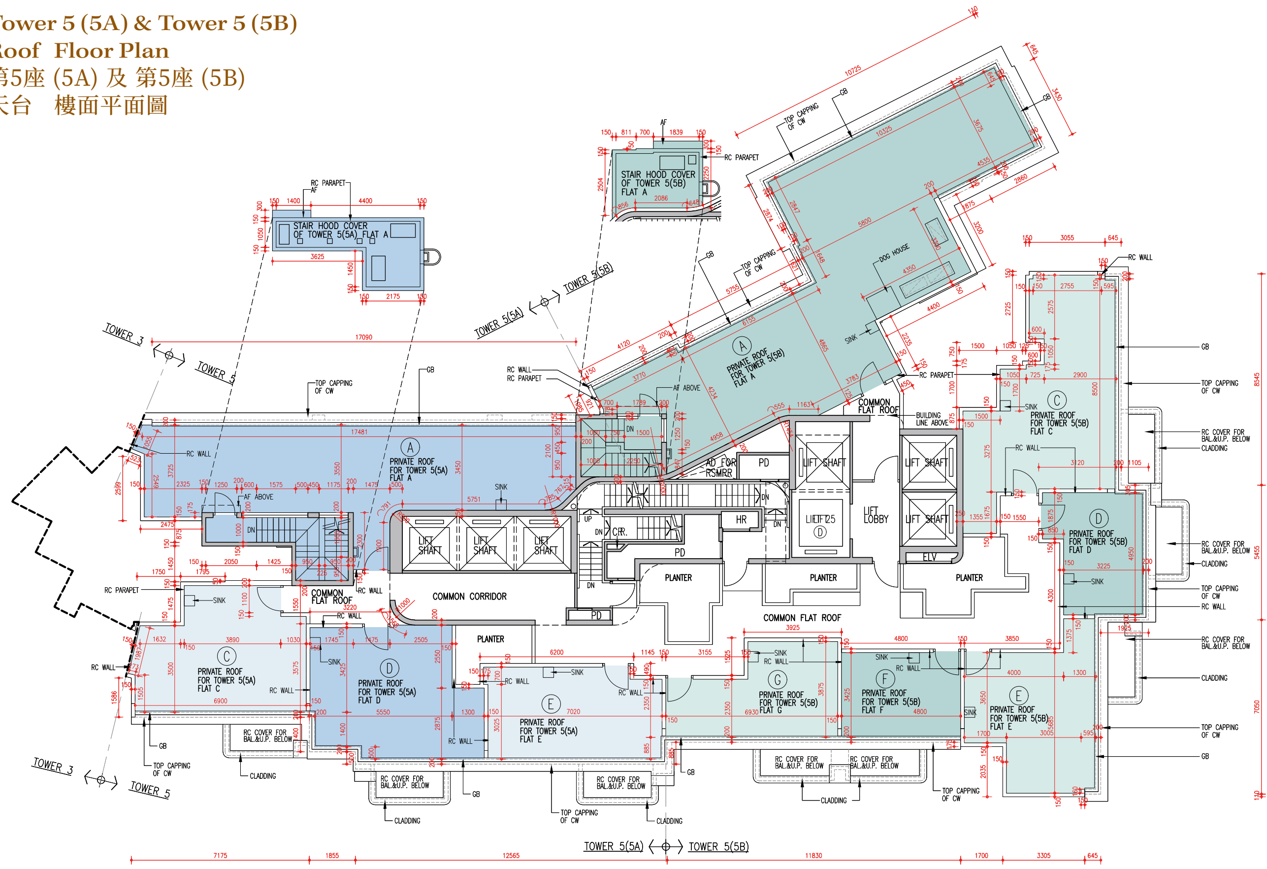
T5 R/F FLOOR PLAN (1 STOREY)
