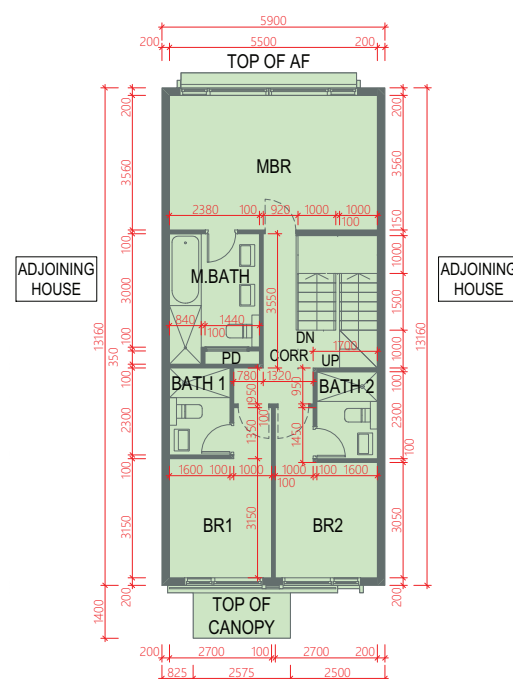
FIRST FLOOR 1樓
