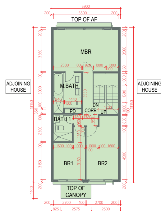
FIRST FLOOR 1樓
