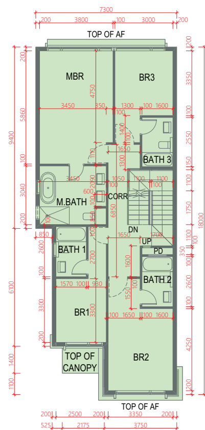
FIRST FLOOR 1樓
