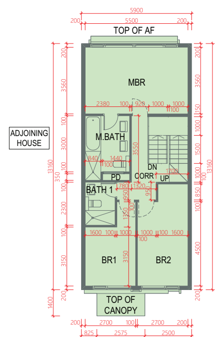
FIRST FLOOR 1樓
