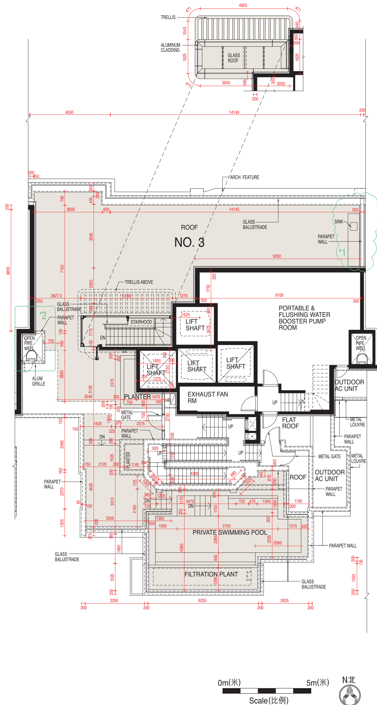
3號現狀間隔平面圖 Floor plan of No.3 showing latest layout
